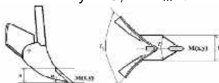
Fig. 2 – Functional parameters of cultivator lister [2]
