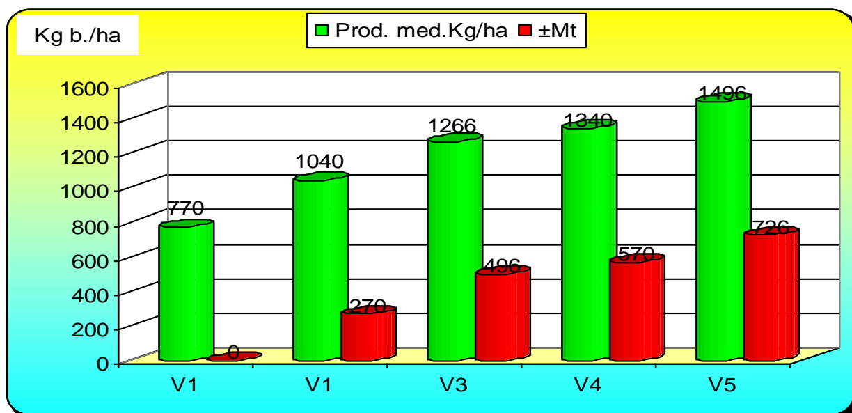
Figure no. 1 . Evolution of production of wheat after mineral and organic fertilization on eutric psamosoil (typical) of the area Poiana Mare (the average grain production(Kg/ha)/2006, 2007, 2008)
